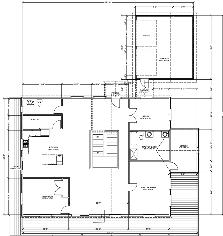
LIVING AREA 2026 sq ft
